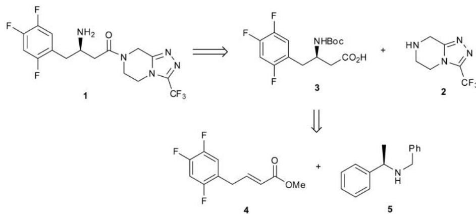
Scheme 1 Strategy for the synthesis of Sitagliptin.
